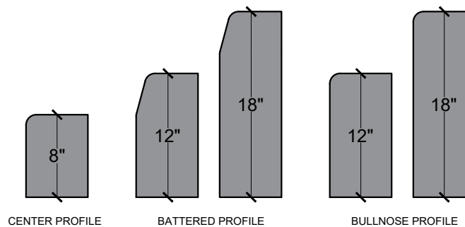
HANOVER® ROCKCURB® PROFILES
